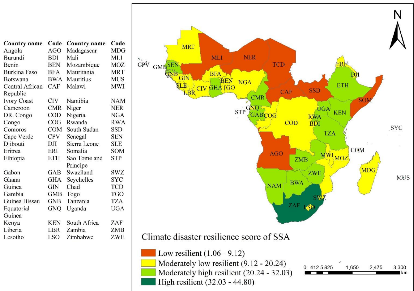
Figure 3. Spatial characteristic of composite national climate resilience index (CNCRI) scores of SSA.
