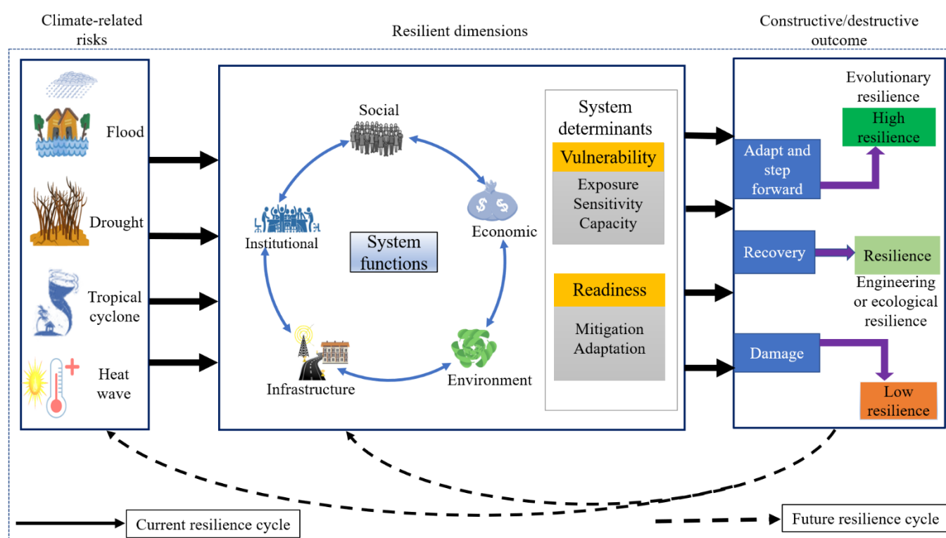
Figure 1. The graphical representation of the climate resilience framework of the study.
